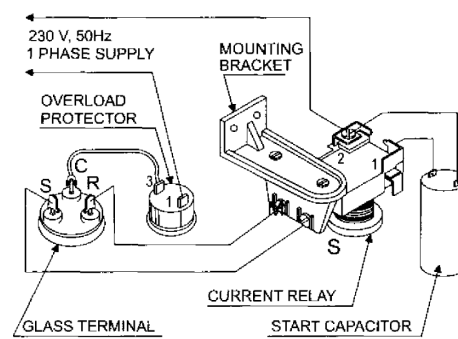
CAPACITOR START INDUCTION RUN (CSIR) WITH CURRENT RELAY
