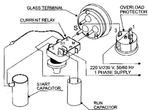
CAPACITOR START CAPACITOR RUN (CSCR) WITH NTC
